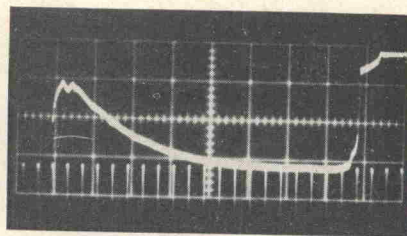
FIG. 21. Manganin gauge in aluminum with peak stress of 30 kilobars.
