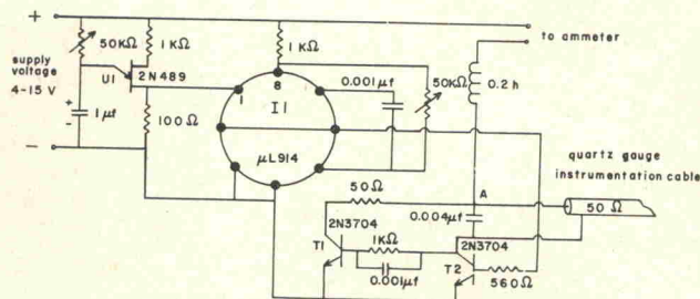
FIG. 19. Diagram of quartz calibration circuit.
